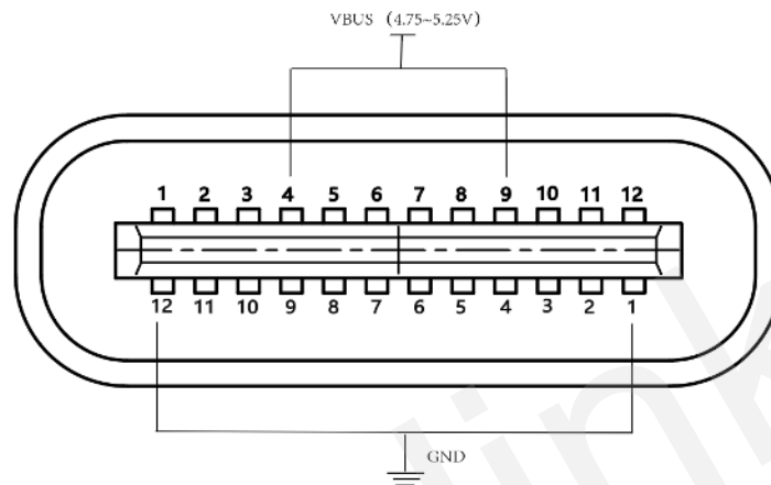
Figure 5. External DC Charger Connection of GL320M
